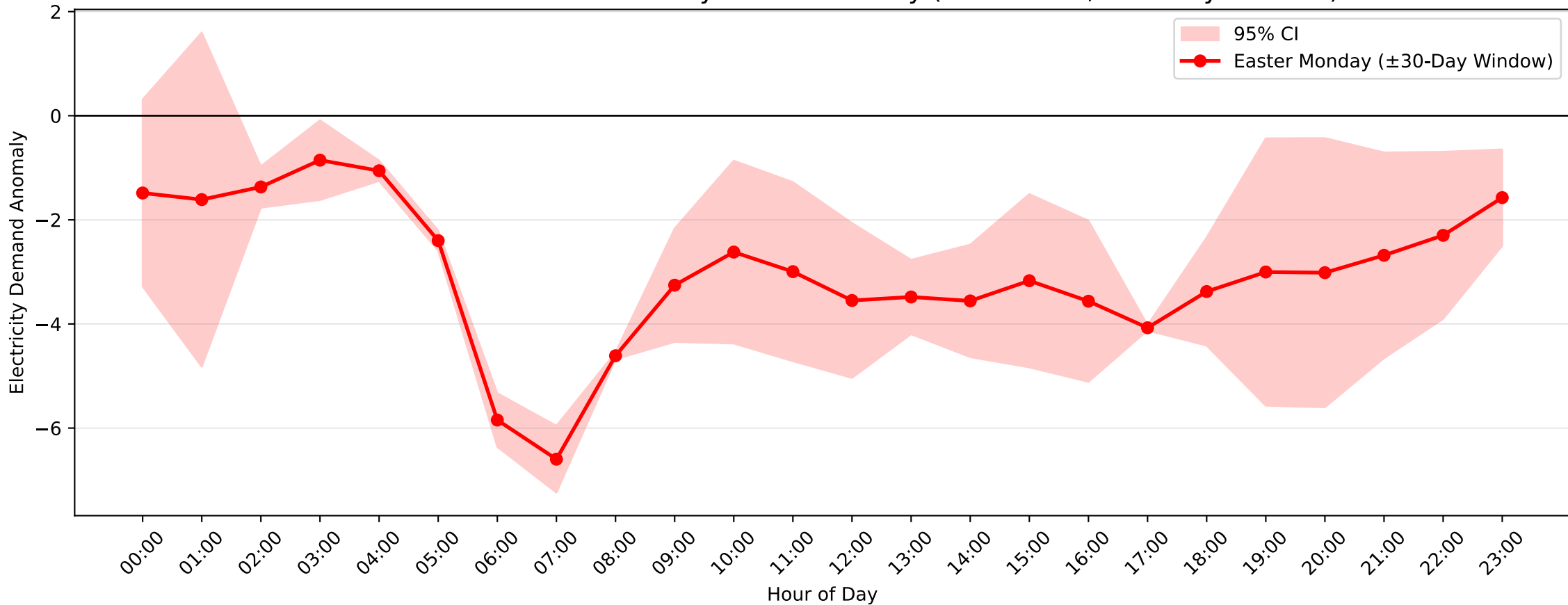
Pennant Hills Demand Anomaly: Easter Monday (2012-2013, \pm 30 -Day Window)
