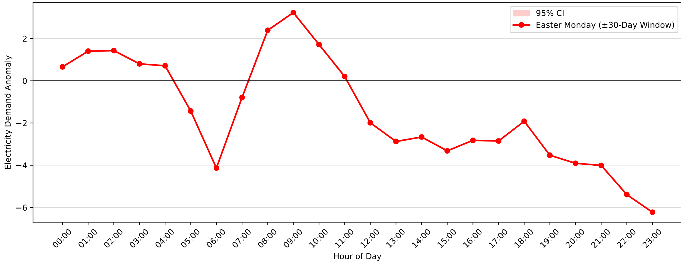
Pennant Hills Demand Anomaly: Easter Monday (2005-2006, \pm 30 -Day Window)
