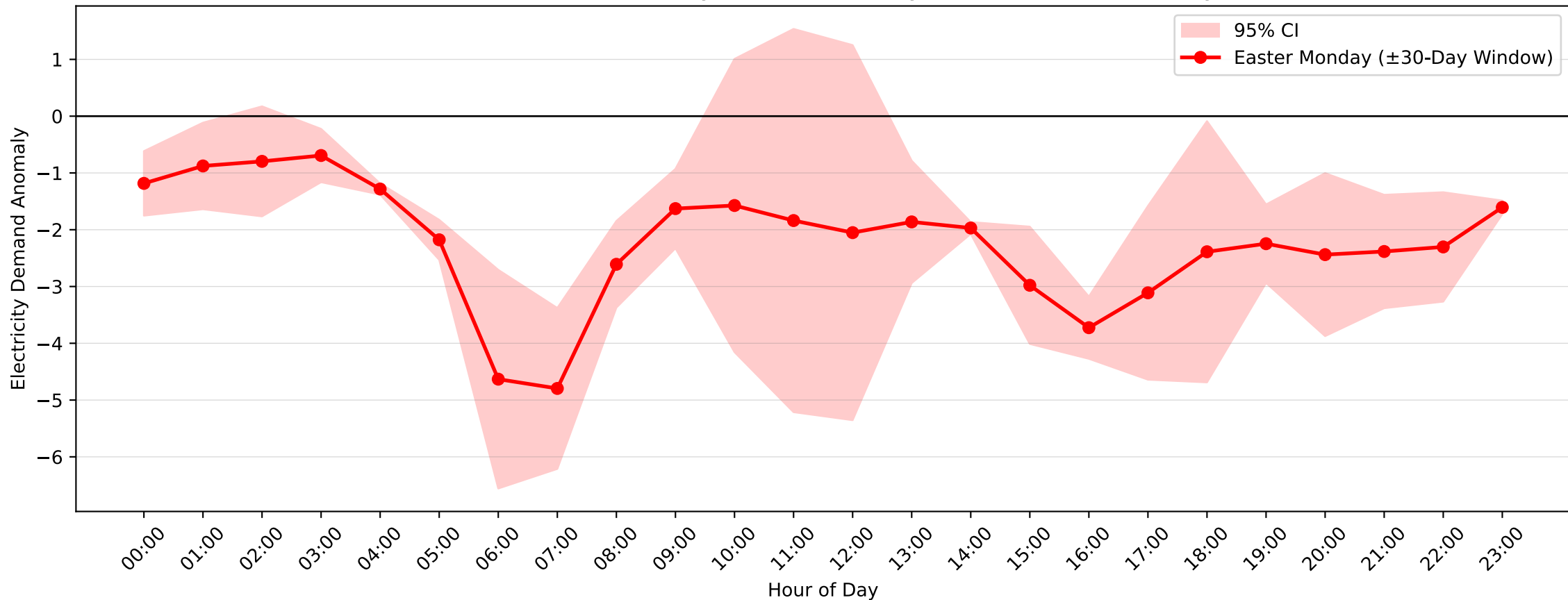
Pennant Hills Demand Anomaly: Easter Monday (2015-2016, \pm 30 -Day Window)
